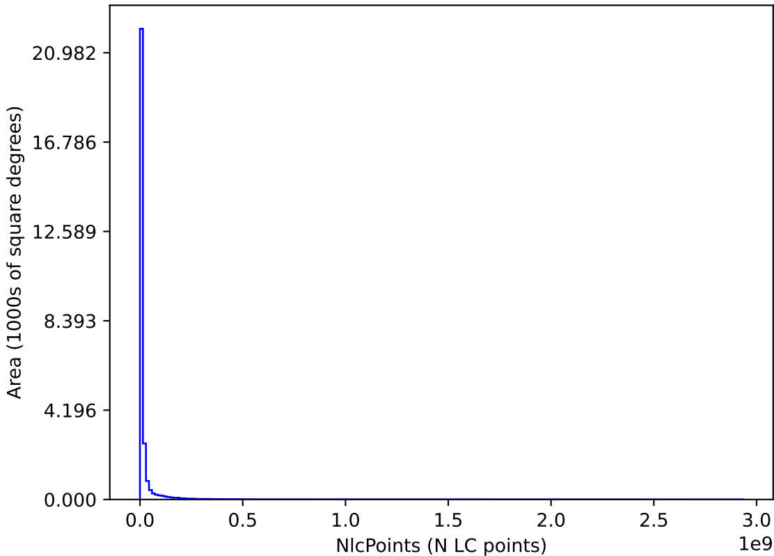
no_long_v3.4_10yrs : NlcPoints
