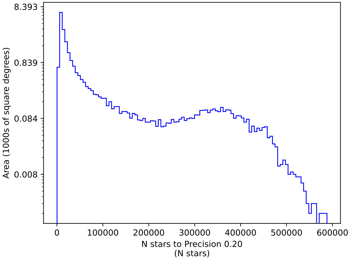
no_long_v3.4_10yrs y: N stars to Precision 0.20
