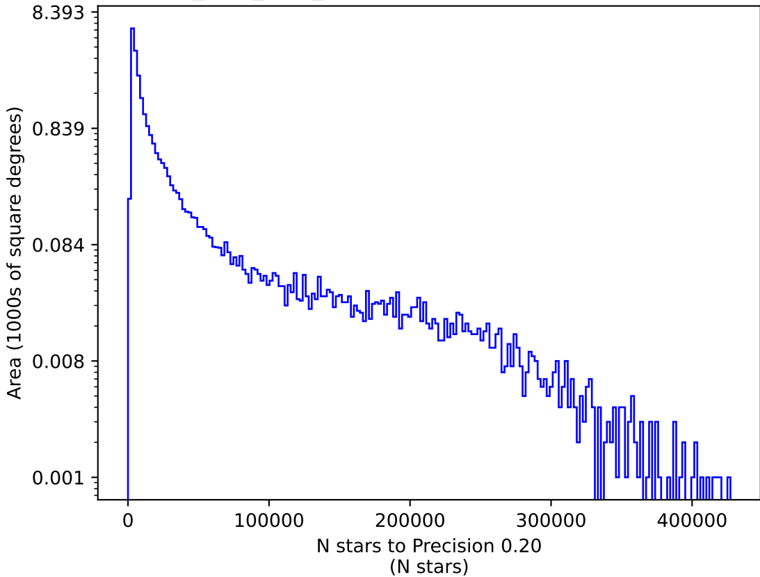
no_long_v3.4_10yrs u: N stars to Precision 0.20
