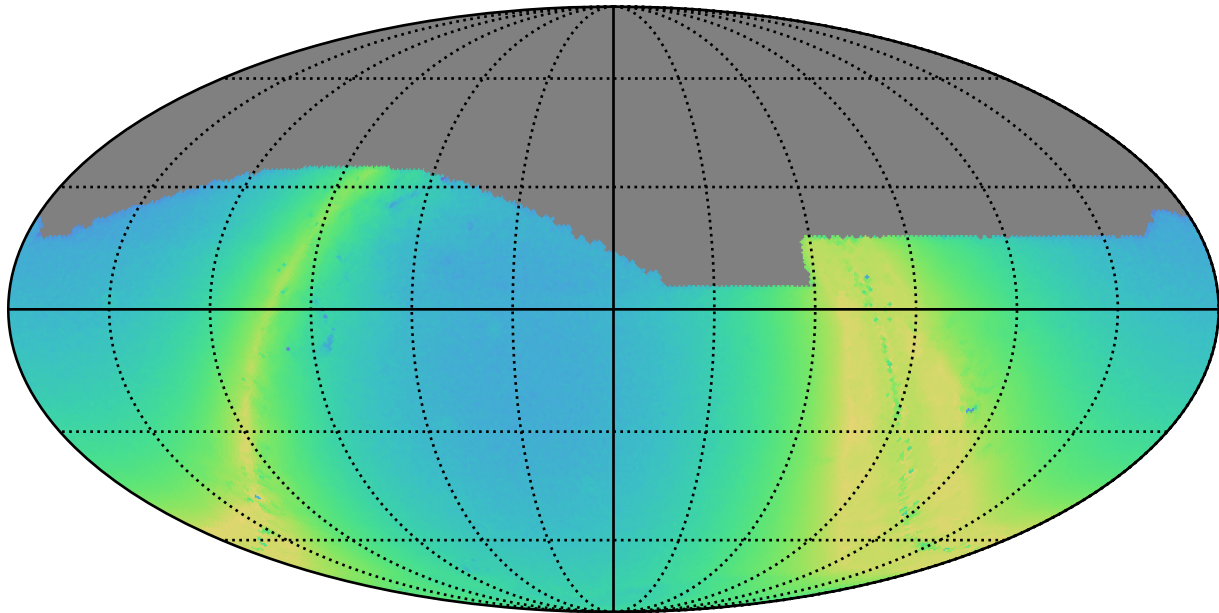
no_long_v3.4_10yrs r: N stars to Precision 0.20
