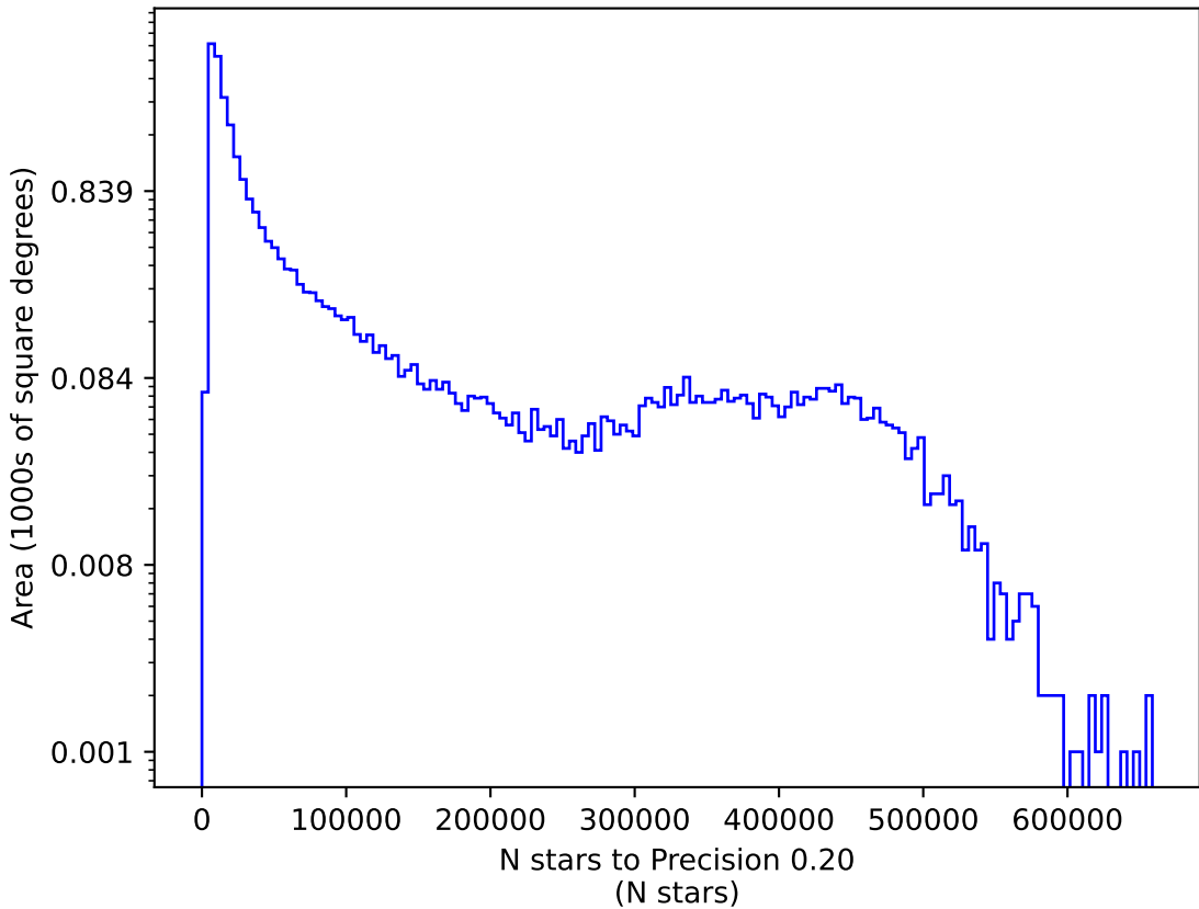
no_long_v3.4_10yrs r: N stars to Precision 0.20
