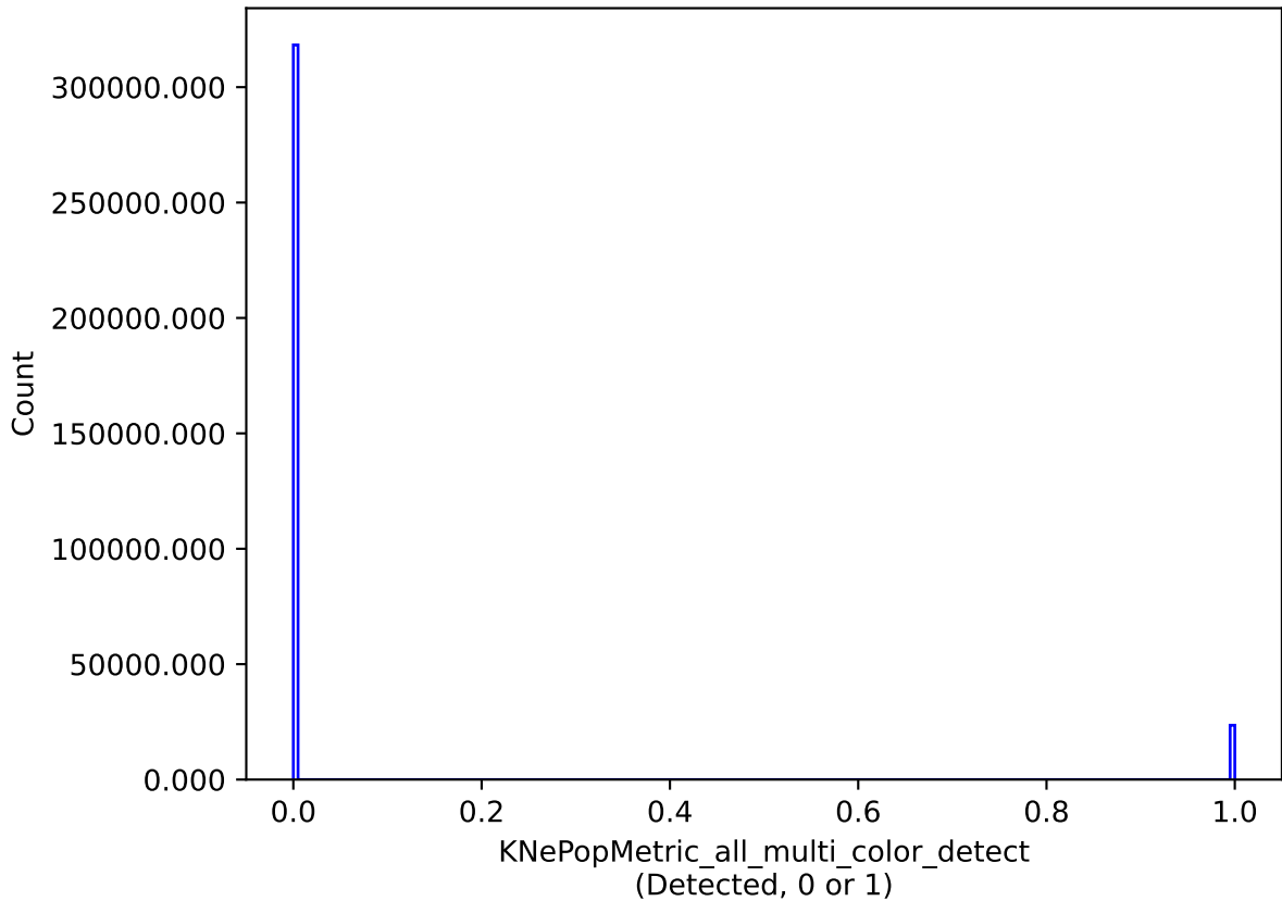
no_long_v3.4_10yrs all models: KNePopMetric_all_multi_color_detect
