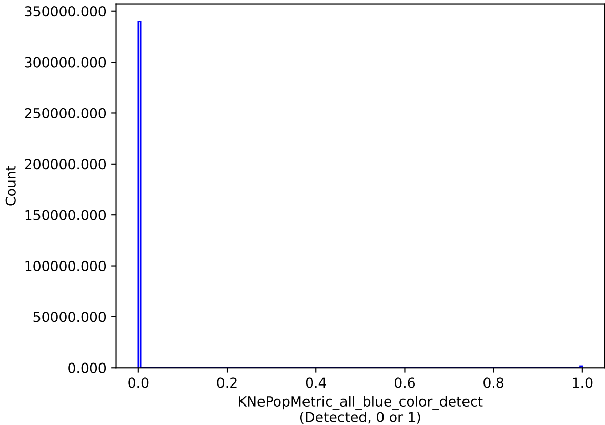
no_long_v3.4_10yrs all models: KNePopMetric_all_blue_color_detect
