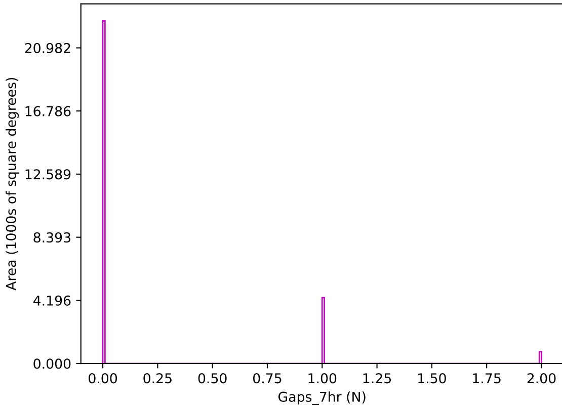
no_long_v3.4_10yrs z band: Gaps_7hr
