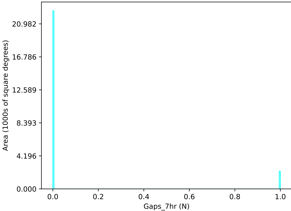
no_long_v3.4_10yrs u band: Gaps_7hr
