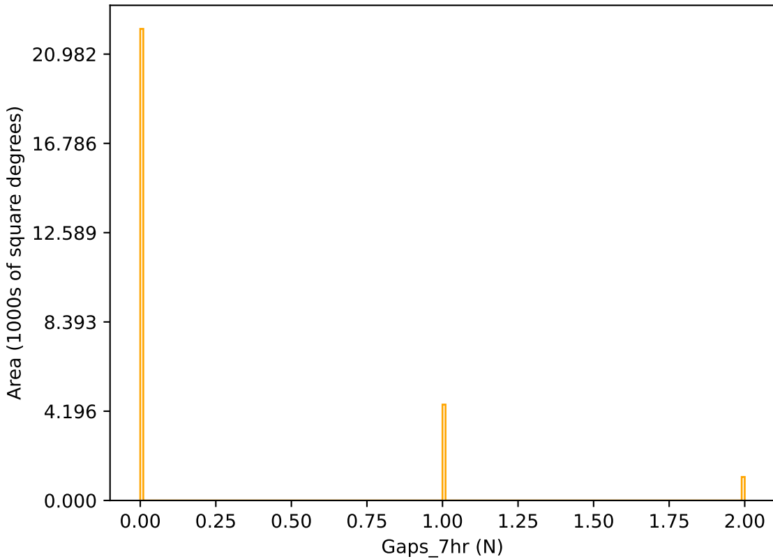
no_long_v3.4_10yrs r band: Gaps_7hr
