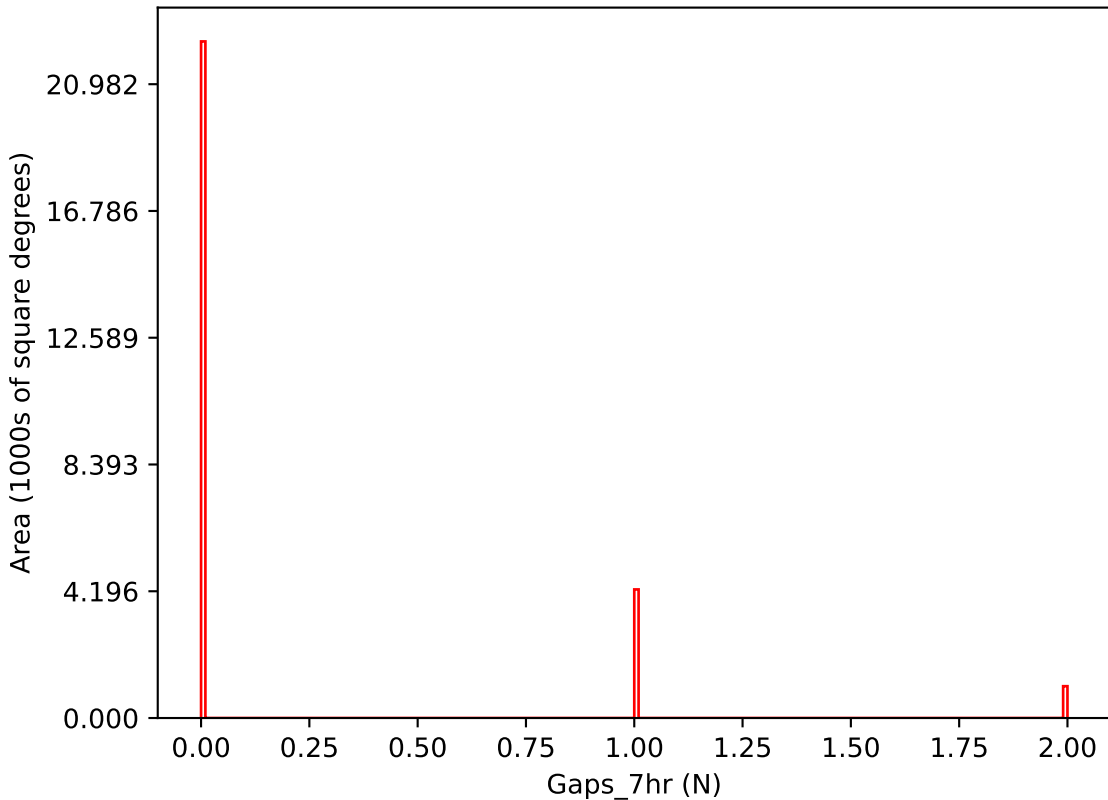
no_long_v3.4_10yrs i band: Gaps_7hr
