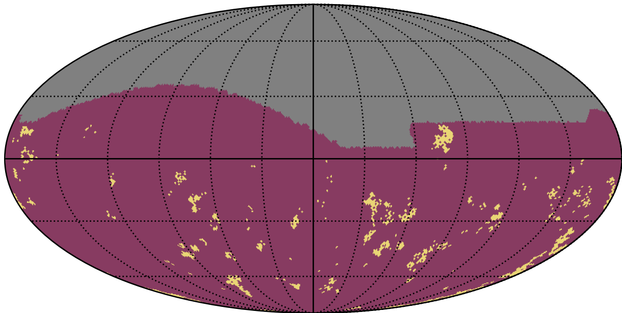
no_long_v3.4_10yrs g band: Gaps_7hr
