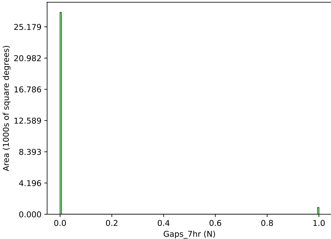
no_long_v3.4_10yrs g band: Gaps_7hr
