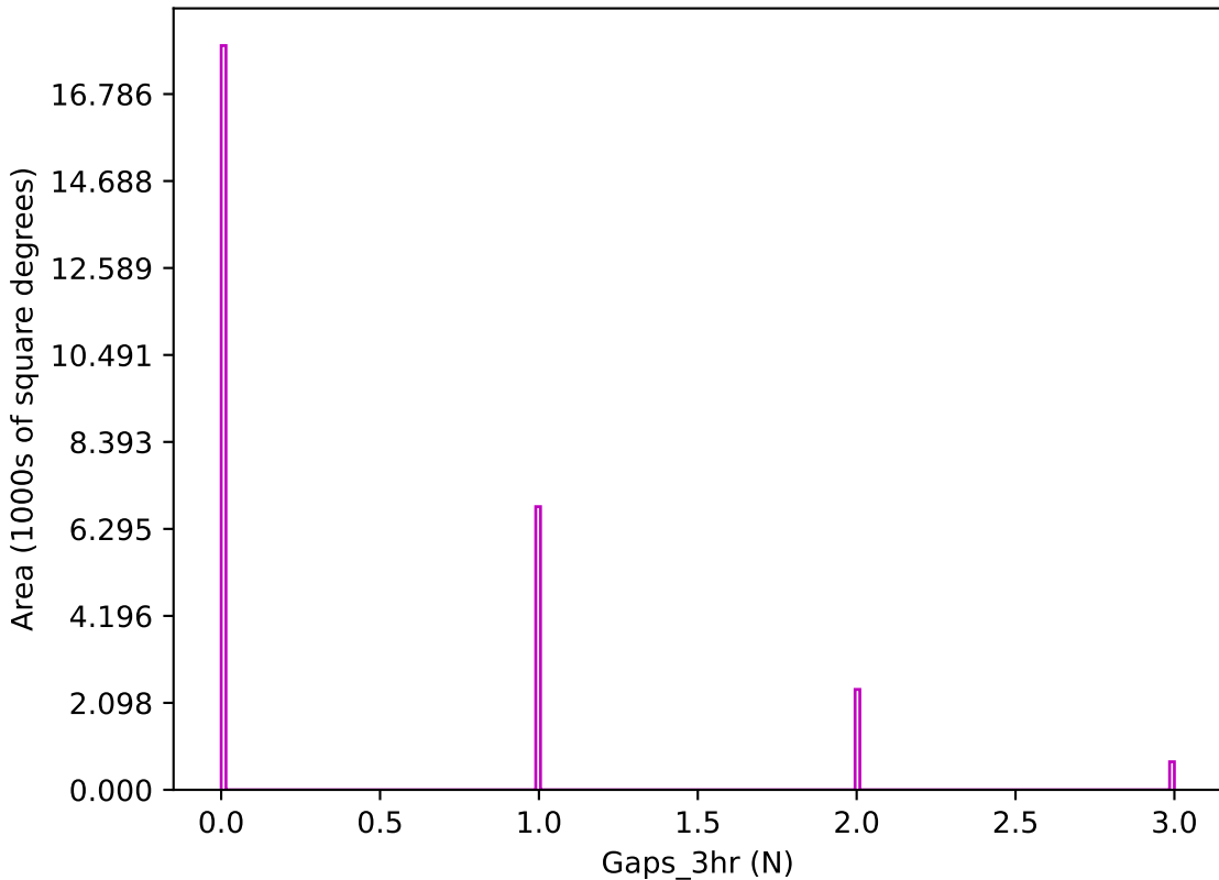
no_long_v3.4_10yrs z band: Gaps_3hr
