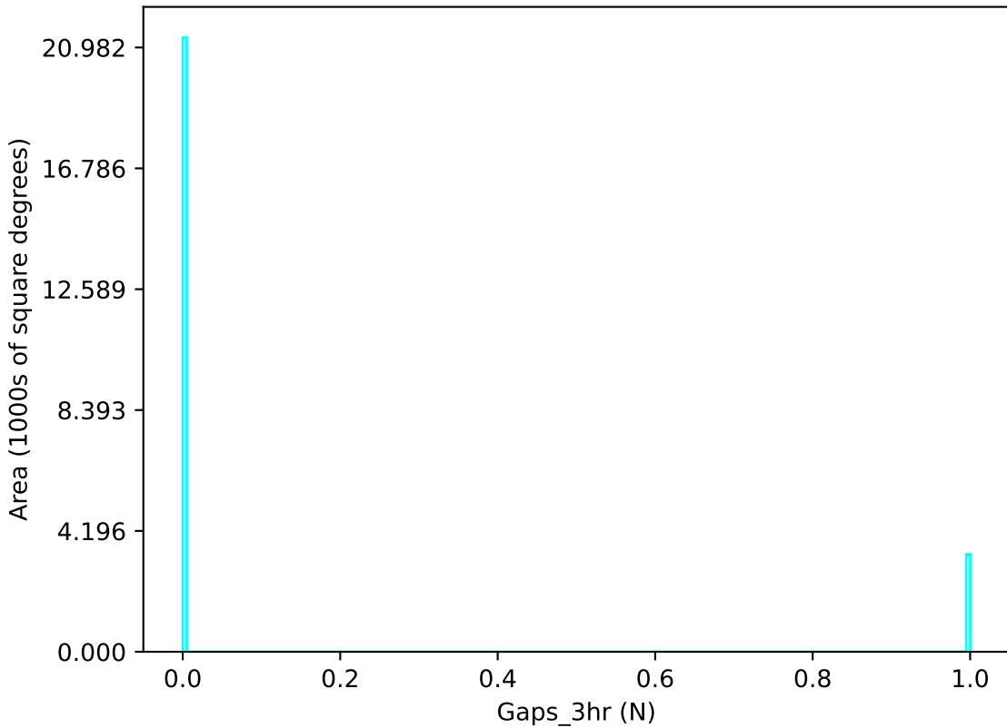
no_long_v3.4_10yrs u band: Gaps_3hr
