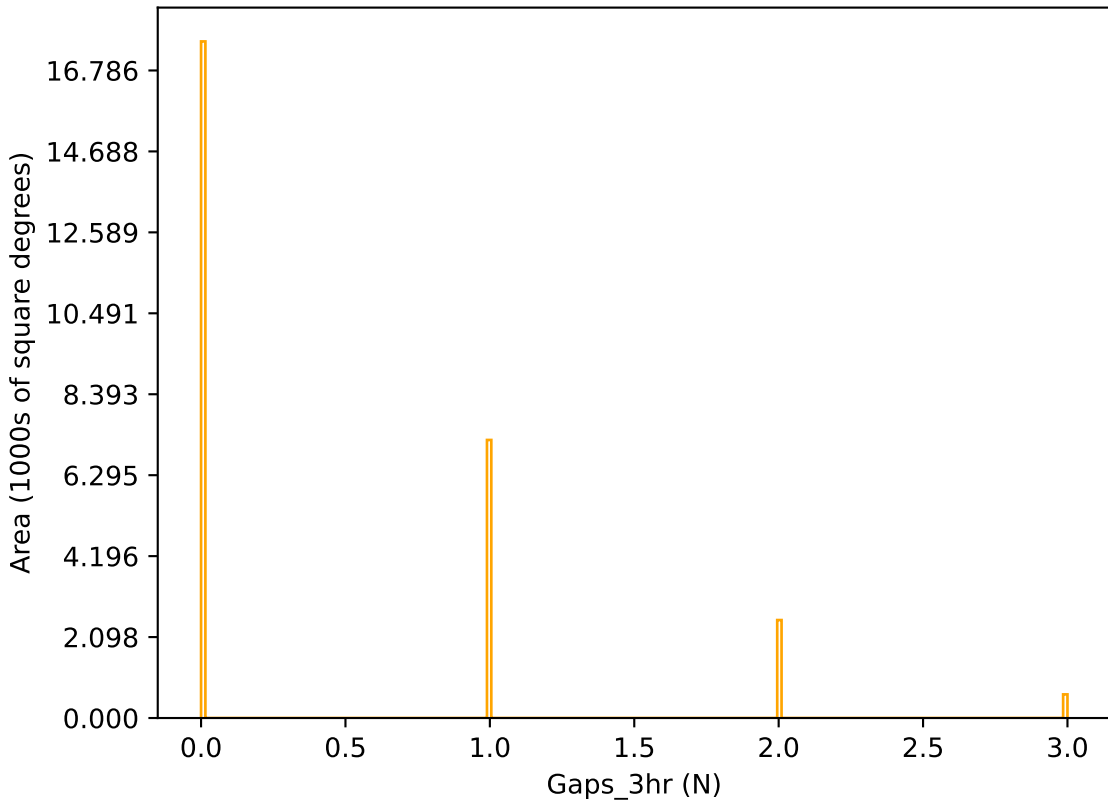
no_long_v3.4_10yrs r band: Gaps_3hr
