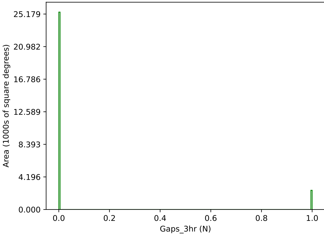
no_long_v3.4_10yrs g band: Gaps_3hr
