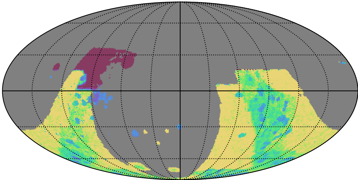
no_long_v3.4_10yrs : GalplaneTimePerFilter_combined_map_y
