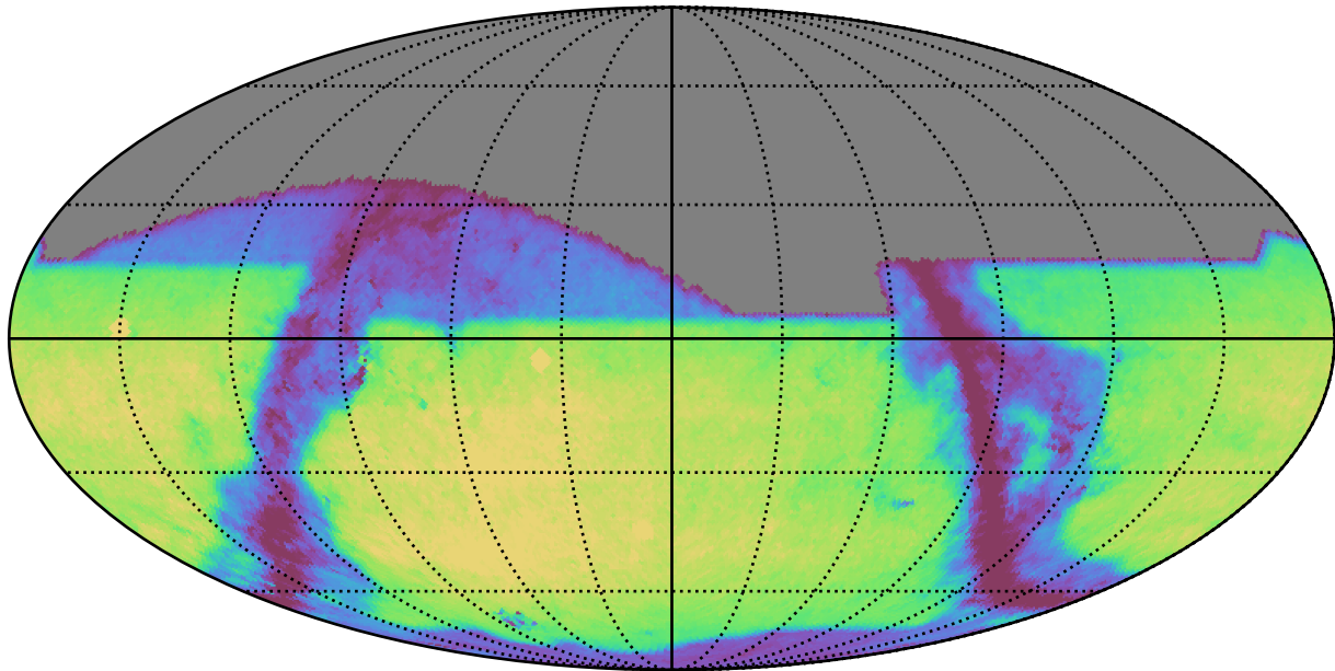
no_long_v3.4_10yrs z: GalaxyCountsMetricExtended
