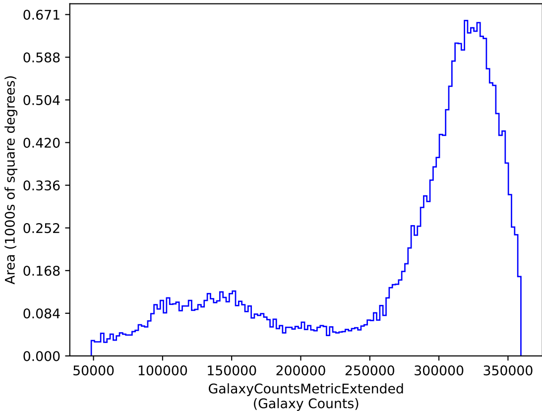
no_long_v3.4_10yrs y: GalaxyCountsMetricExtended
