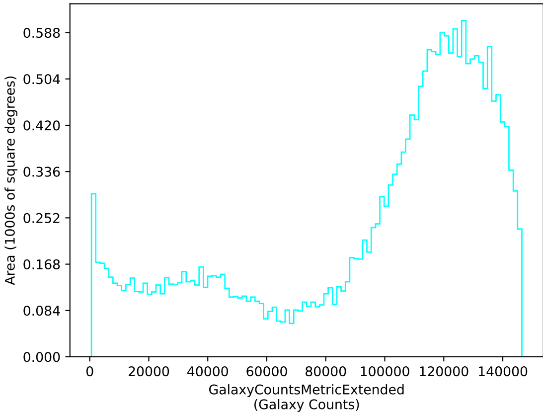
no_long_v3.4_10yrs u: GalaxyCountsMetricExtended
