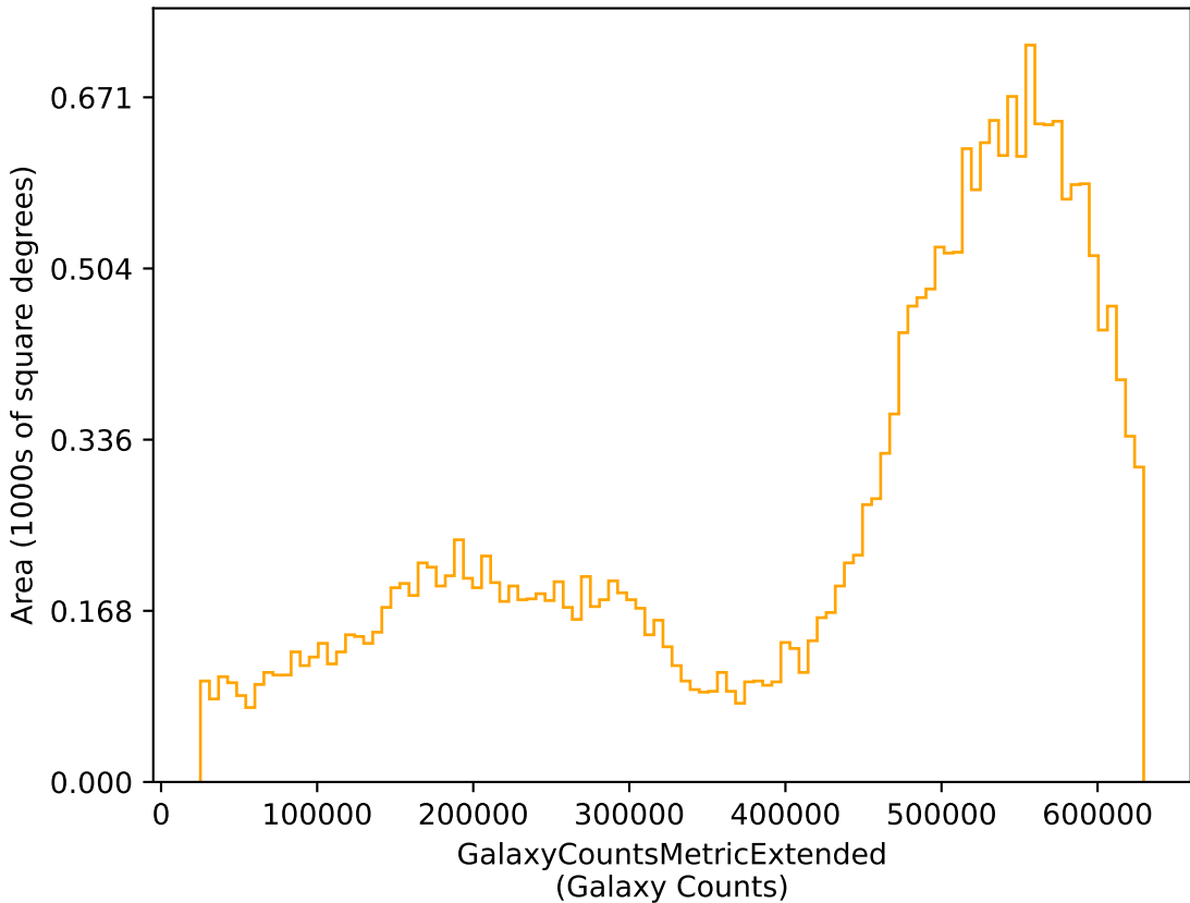
no_long_v3.4_10yrs r: GalaxyCountsMetricExtended
