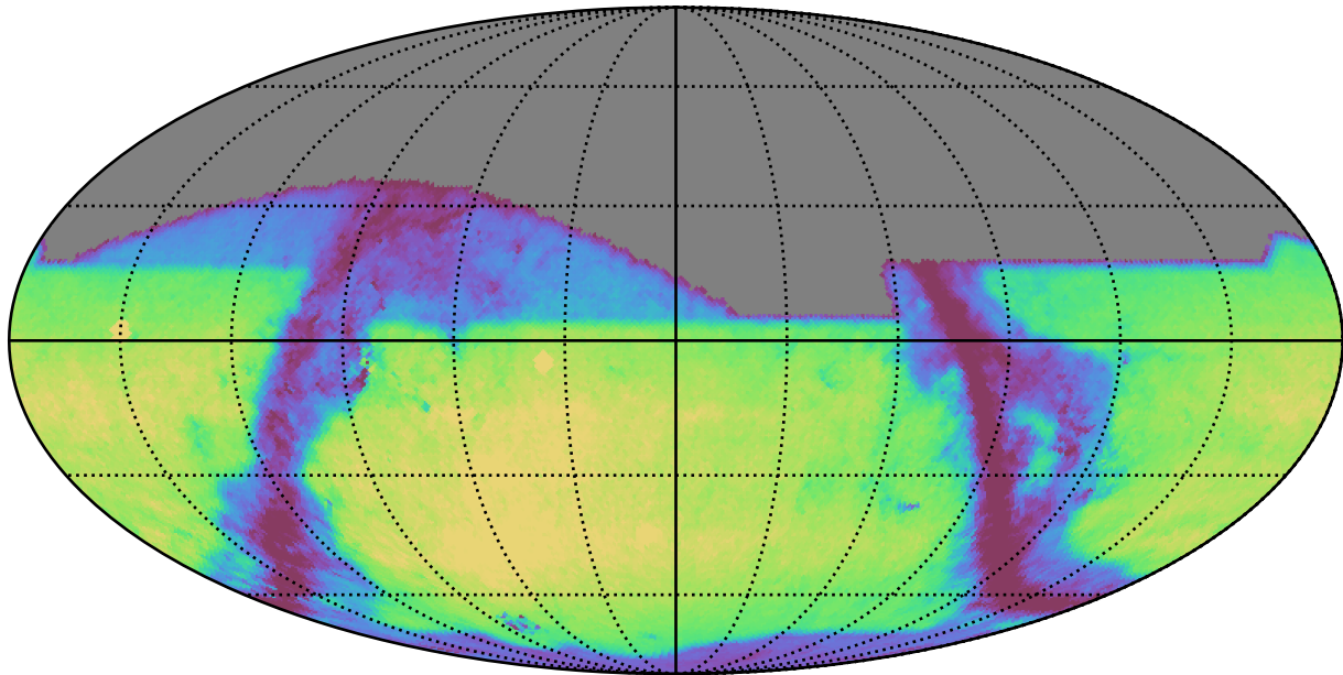
no_long_v3.4_10yrs i: GalaxyCountsMetricExtended
