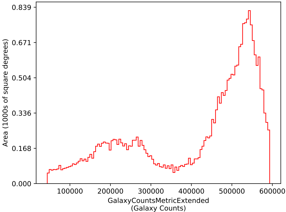
no_long_v3.4_10yrs i: GalaxyCountsMetricExtended
