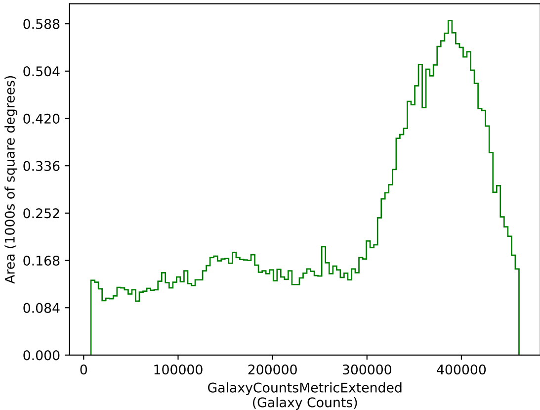
no_long_v3.4_10yrs g: GalaxyCountsMetricExtended
