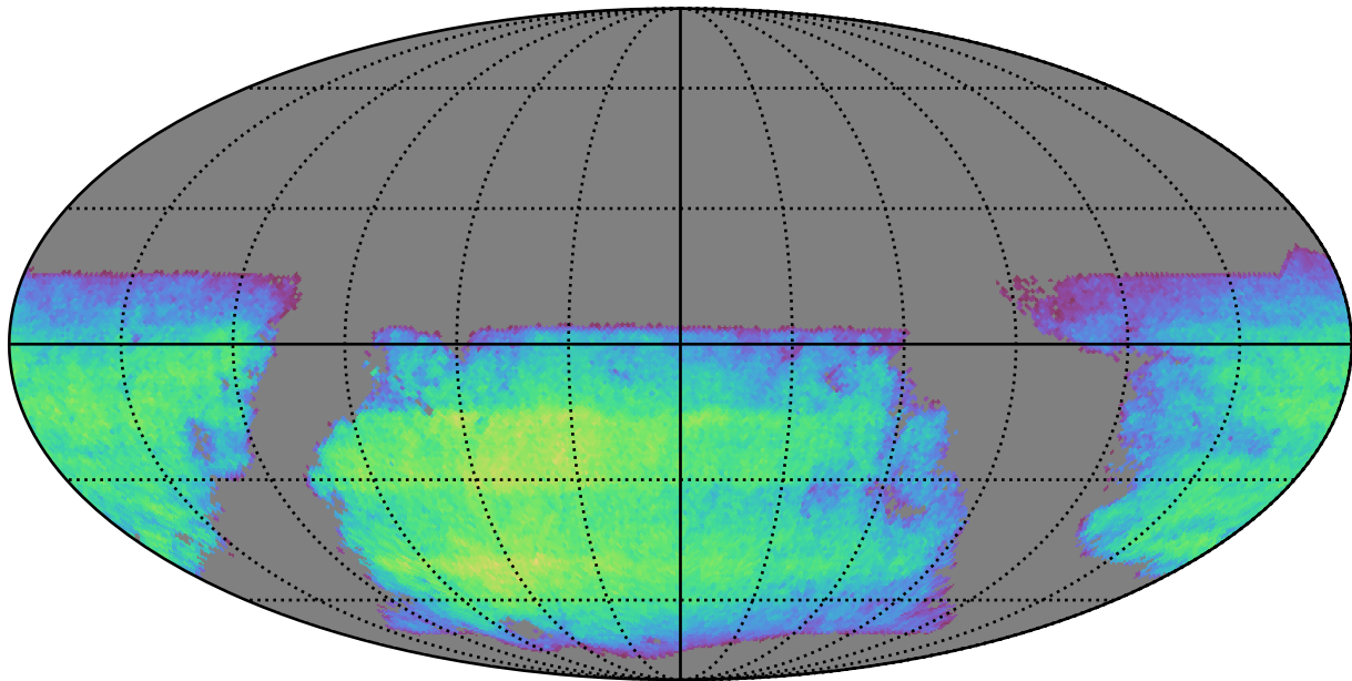
no_long_v3.4_10yrs i band non-DD year 9: ExgalM5WithCuts
