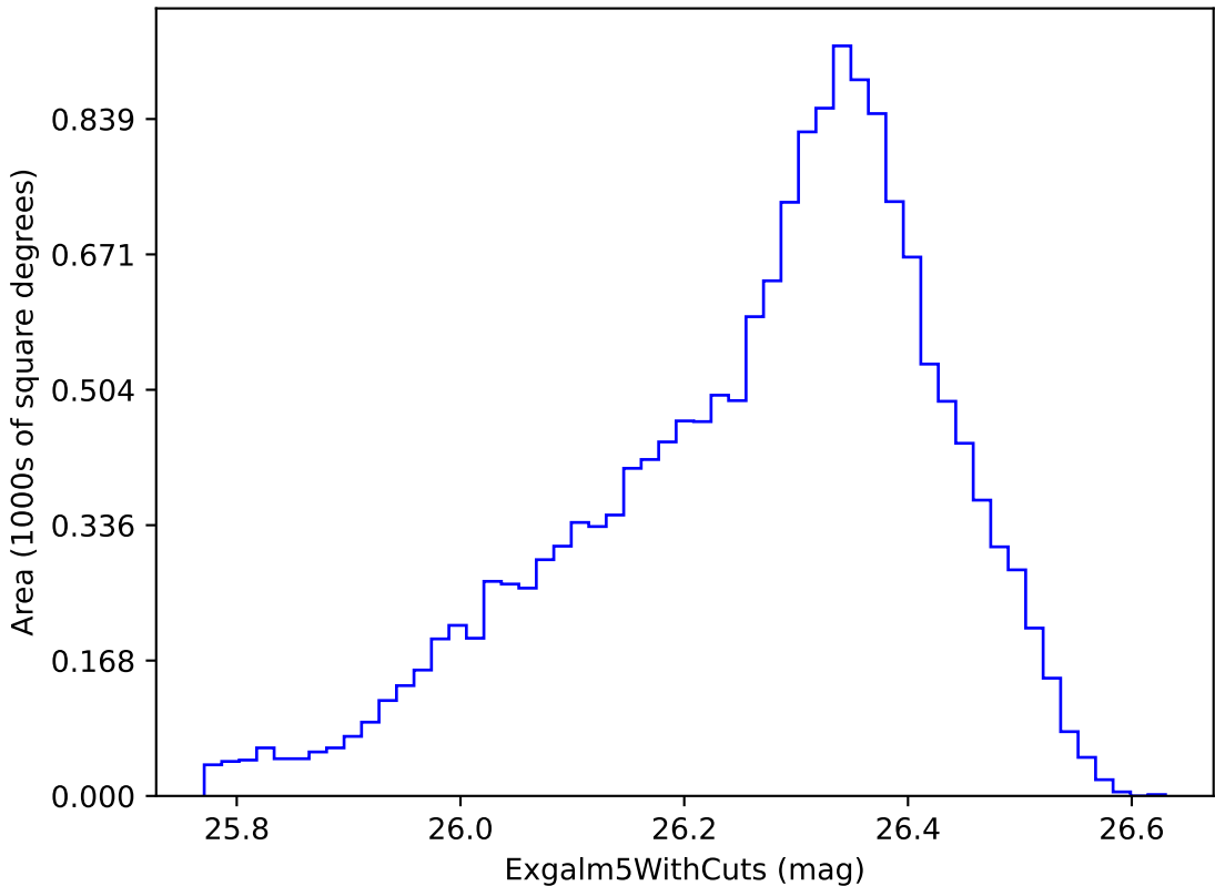
no_long_v3.4_10yrs i band non-DD year 8: ExgalM5WithCuts
