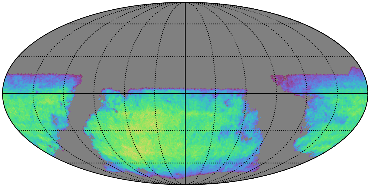
no_long_v3.4_10yrs i band non-DD year 6: ExgalM5WithCuts
