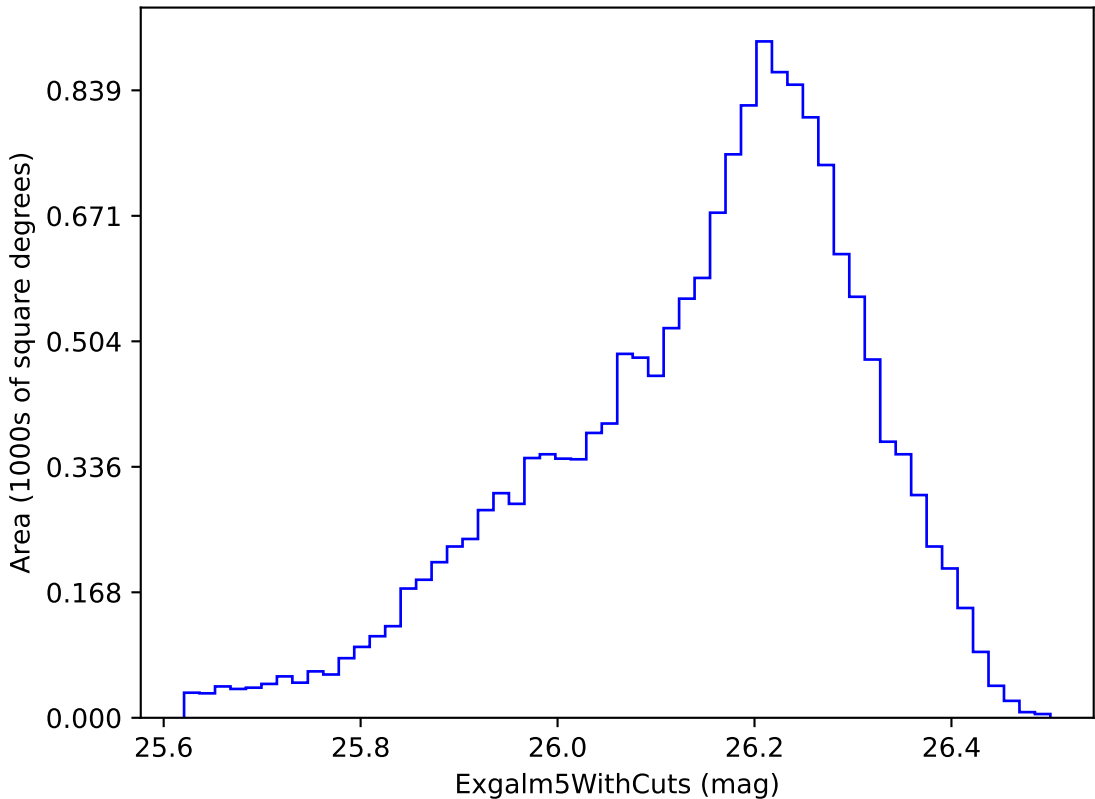
no_long_v3.4_10yrs i band non-DD year 6: ExgalM5WithCuts
