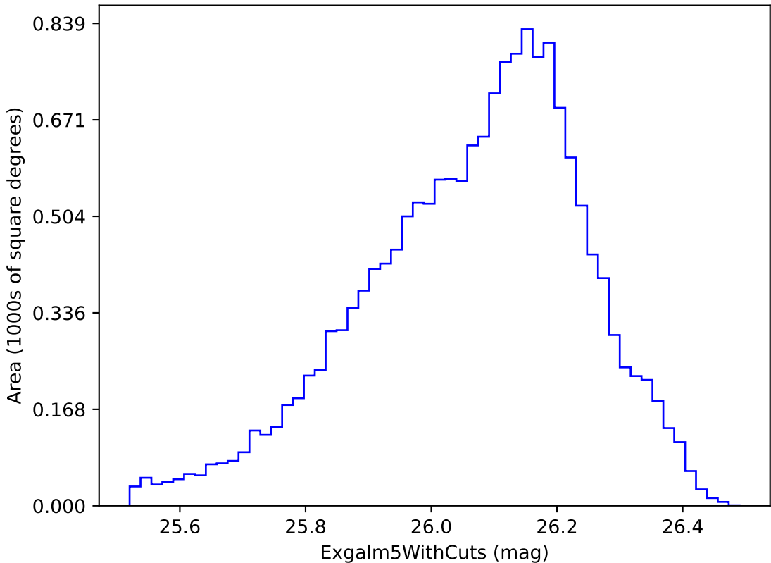
no_long_v3.4_10yrs i band non-DD year 5: ExgalM5WithCuts
