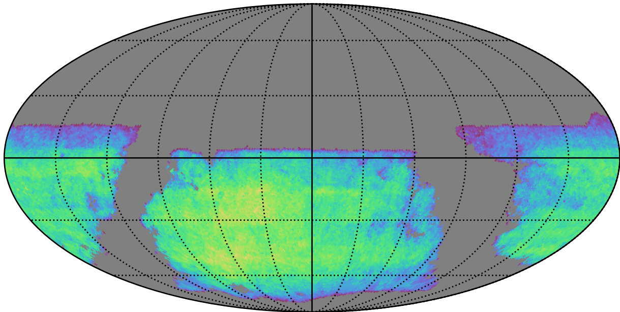
no_long_v3.4_10yrs i band non-DD year 4: ExgalM5WithCuts
