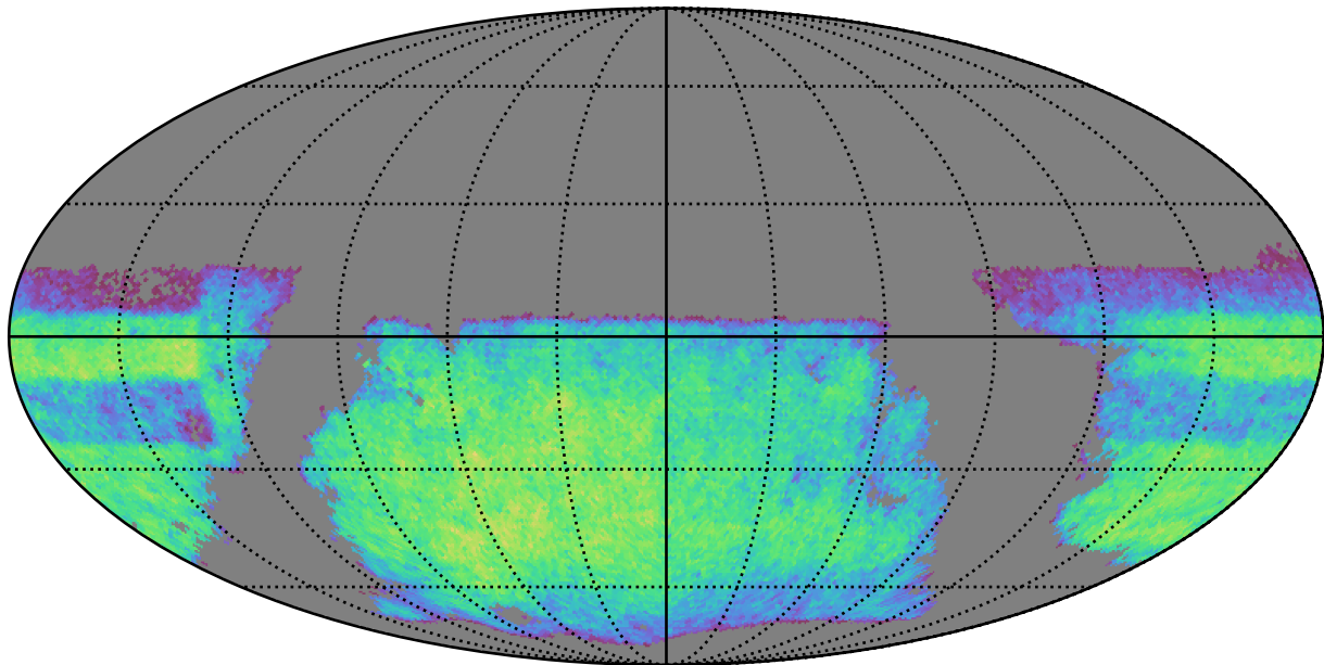
no_long_v3.4_10yrs i band non-DD year 2: ExgalM5WithCuts
