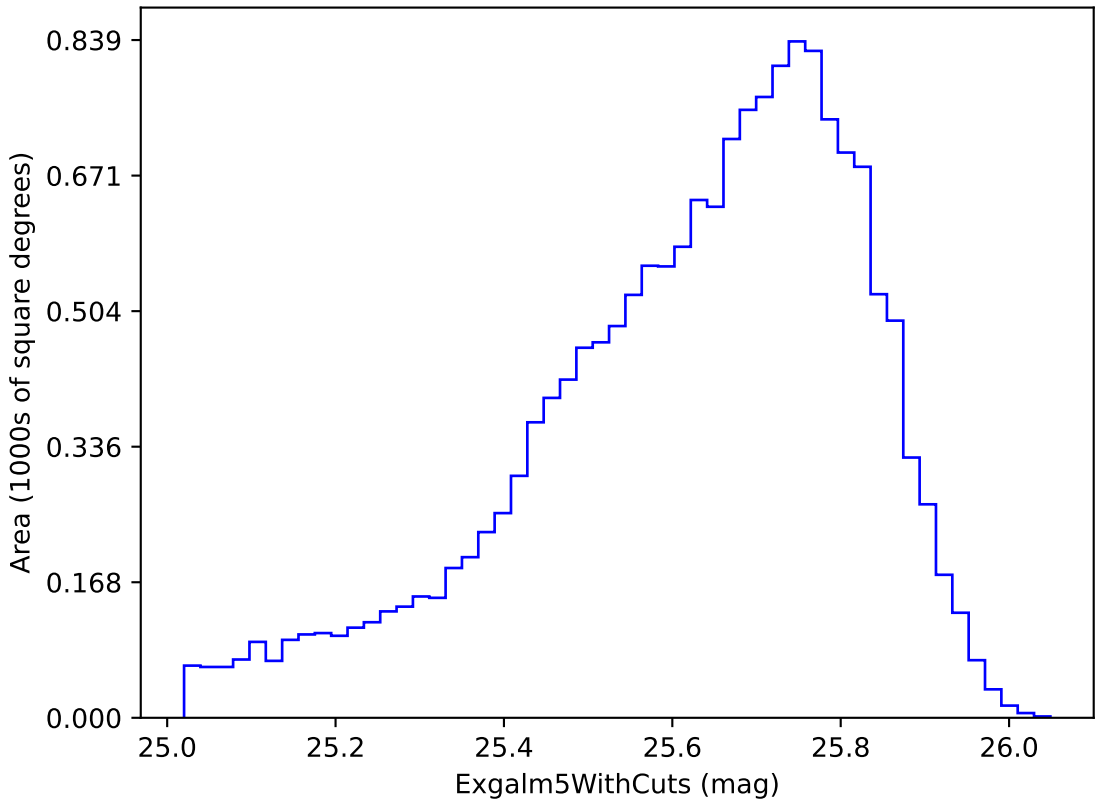
no_long_v3.4_10yrs i band non-DD year 2: ExgalM5WithCuts
