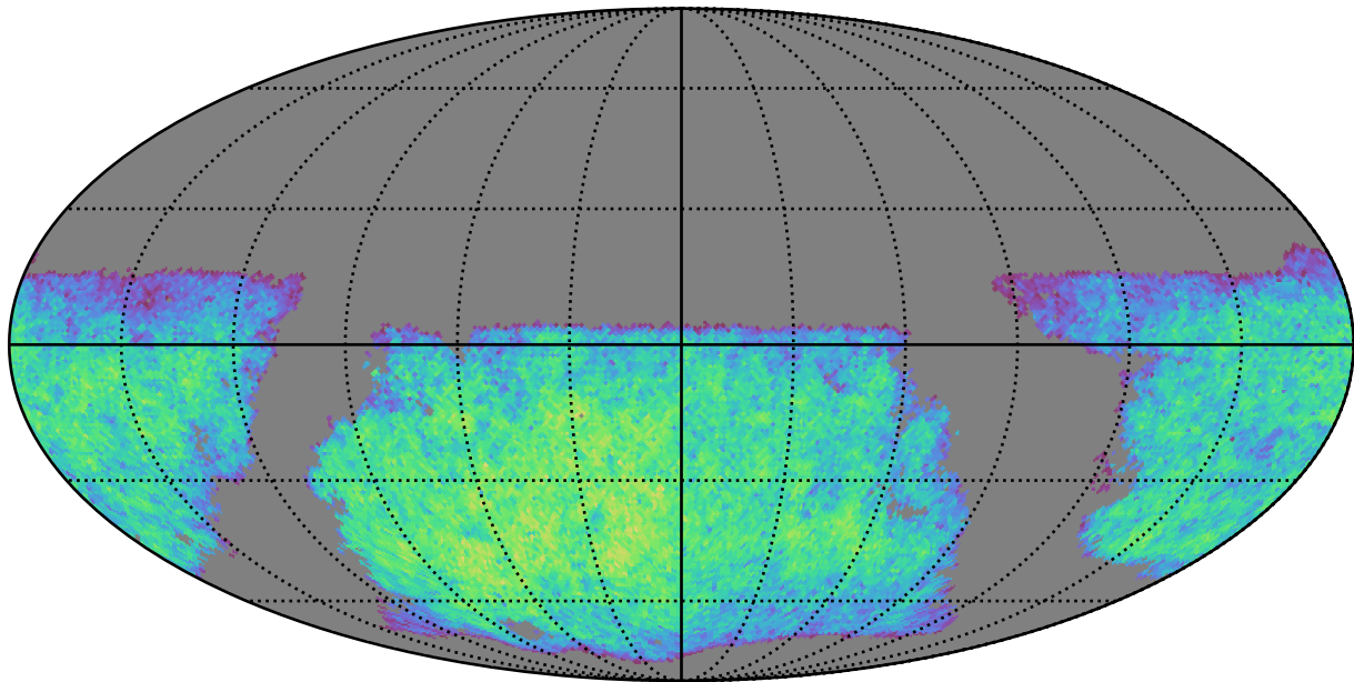
no_long_v3.4_10yrs i band non-DD year 1: ExgalM5WithCuts
