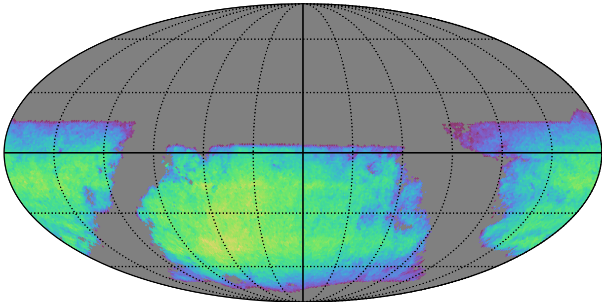
no_long_v3.4_10yrs i band non-DD year 10: ExgalM5WithCuts
