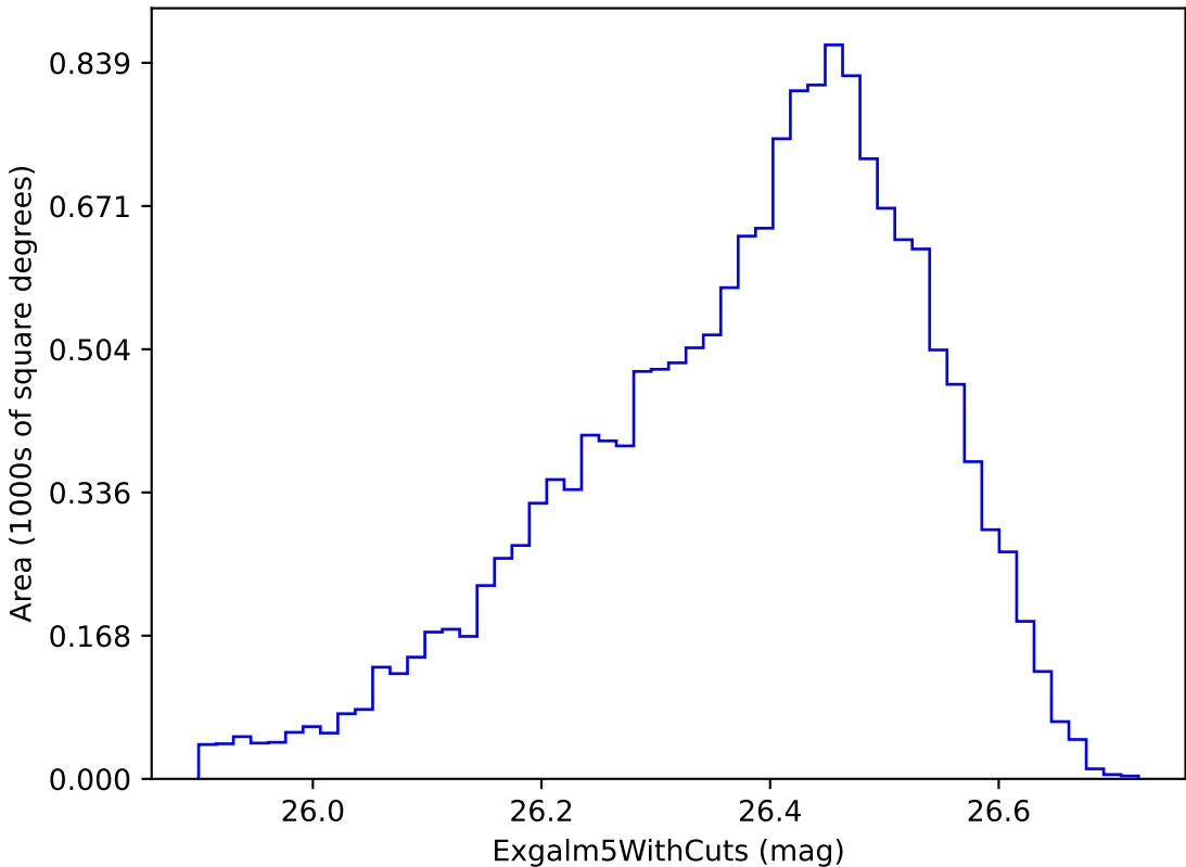
no_long_v3.4_10yrs i band non-DD year 10: ExgalM5WithCuts
