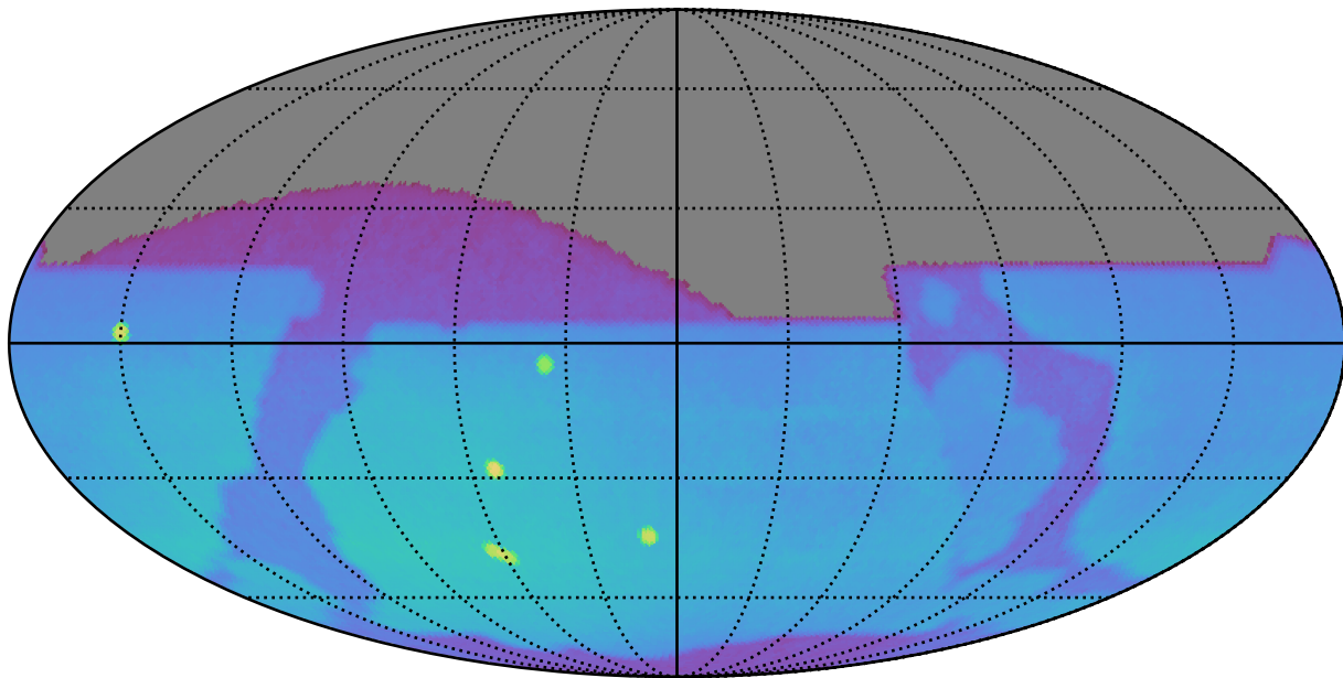
no_long_v3.4_10yrs : Brown Dwarf, L7
