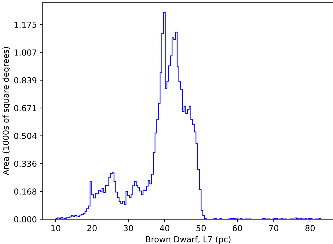
no_long_v3.4_10yrs : Brown Dwarf, L7
