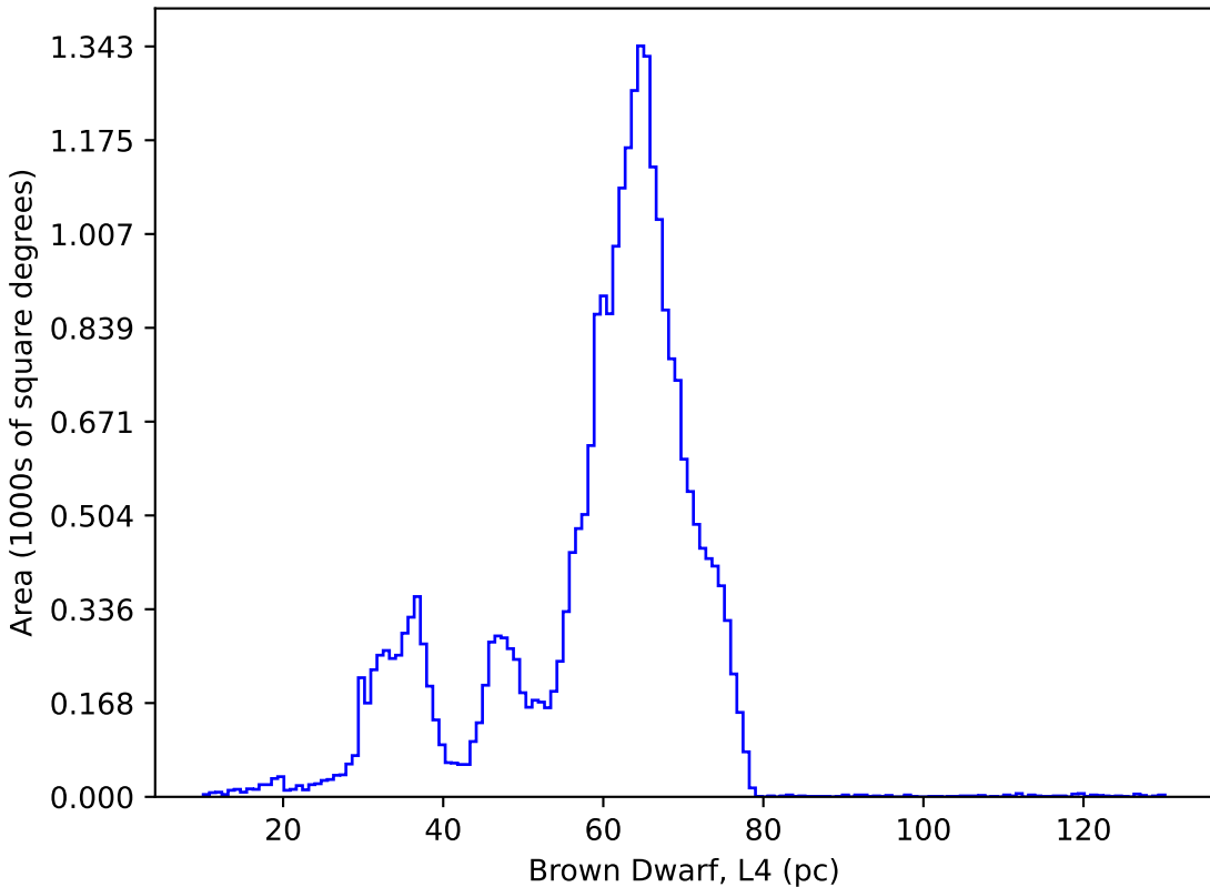
no_long_v3.4_10yrs : Brown Dwarf, L4
