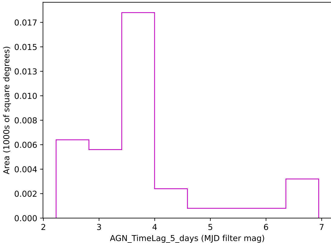
no_long_v3.4_10yrs z band: AGN_TimeLag_5_days
