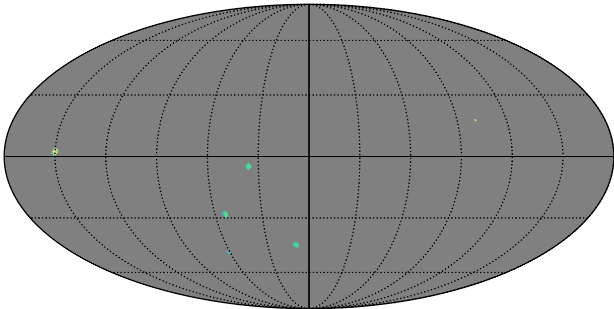
no_long_v3.4_10yrs r band: AGN_TimeLag_5_days
