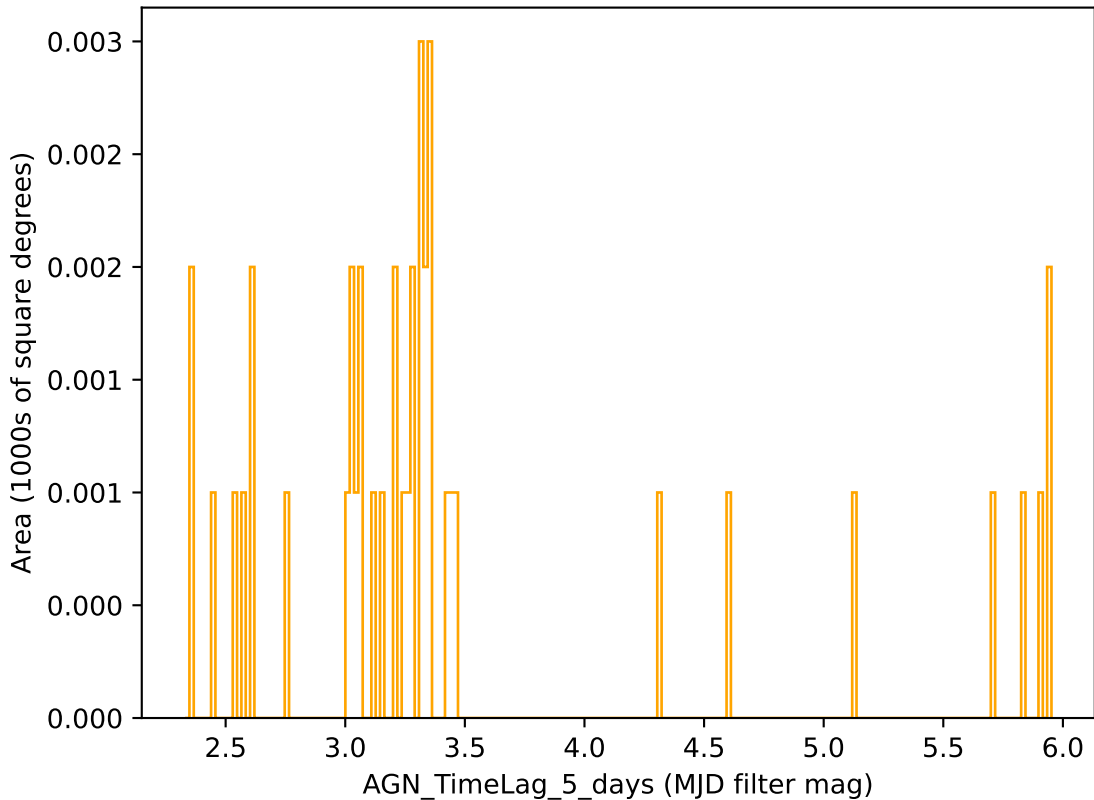
no_long_v3.4_10yrs r band: AGN_TimeLag_5_days
