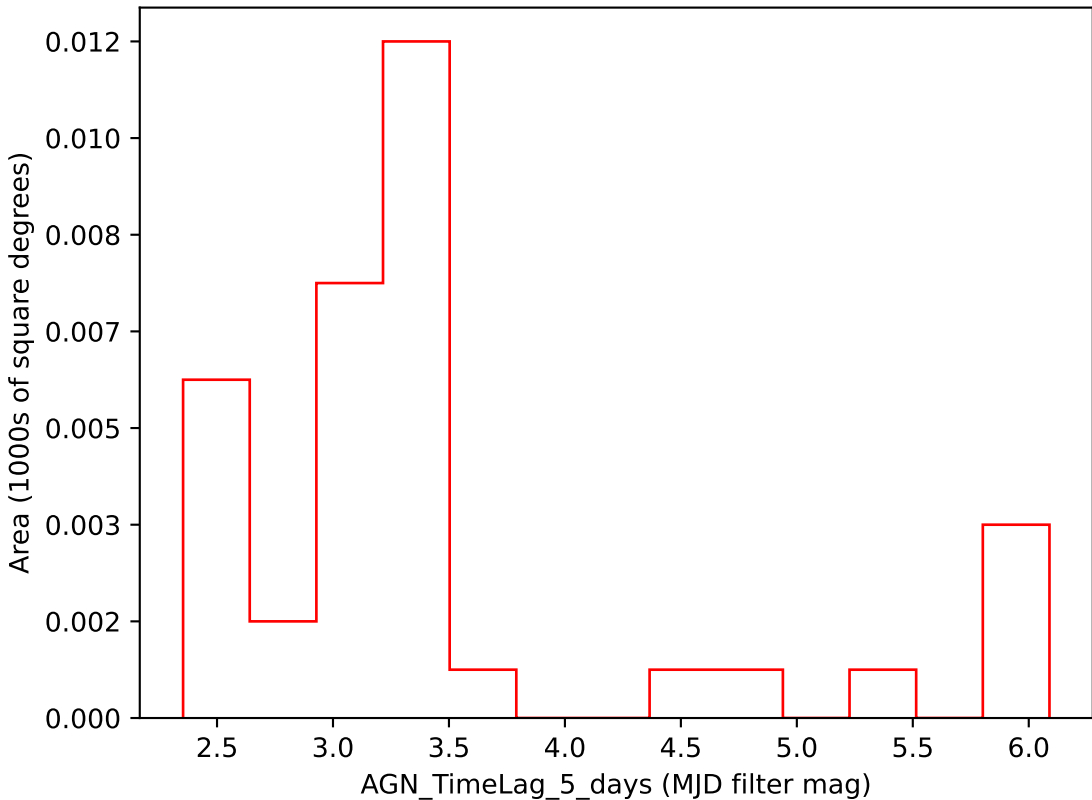
no_long_v3.4_10yrs i band: AGN_TimeLag_5_days
