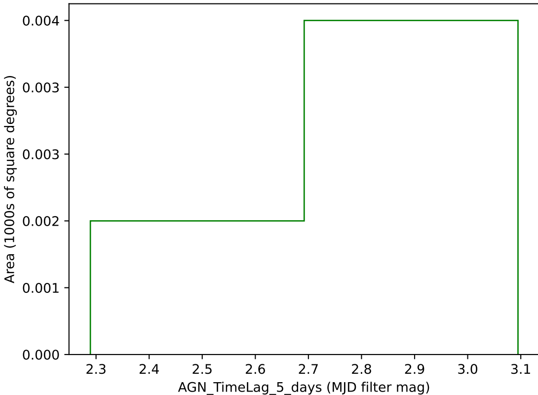
no_long_v3.4_10yrs g band: AGN_TimeLag_5_days
