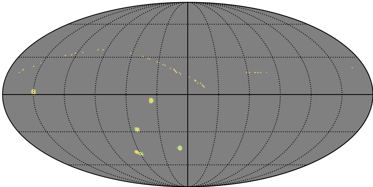
no_long_v3.4_10yrs all bands: AGN_TimeLag_5_days
