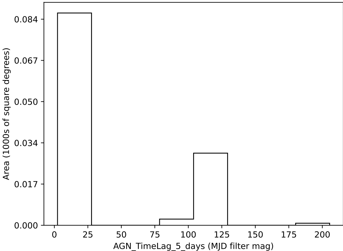
no_long_v3.4_10yrs all bands: AGN_TimeLag_5_days
