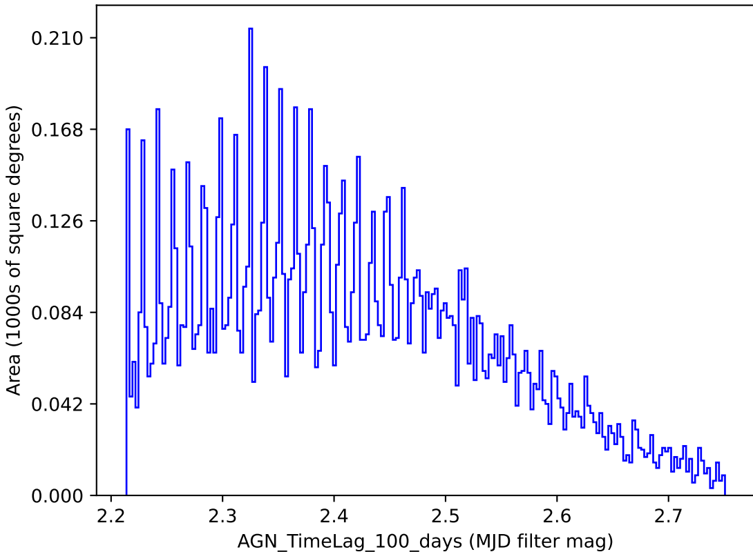
no_long_v3.4_10yrs y band: AGN_TimeLag_100_days
