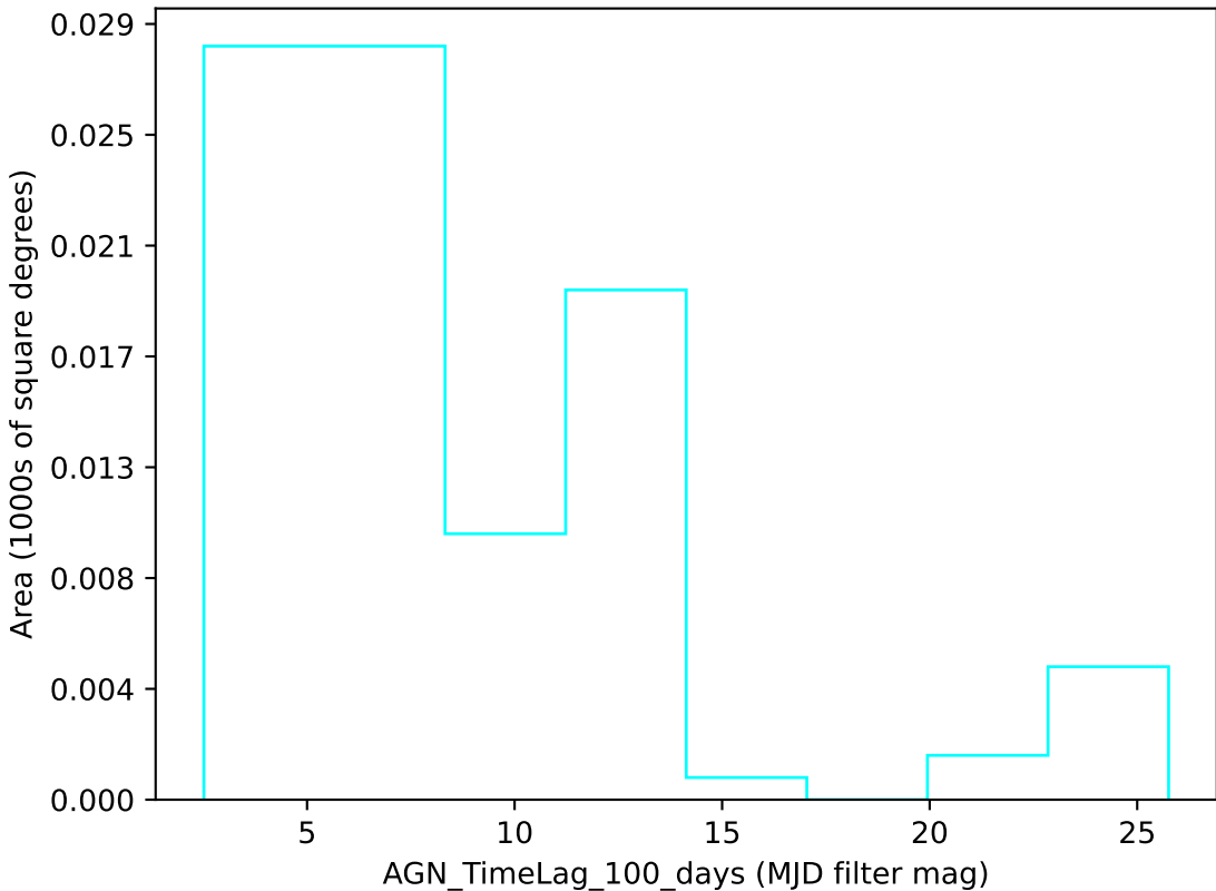
no_long_v3.4_10yrs u band: AGN_TimeLag_100_days
