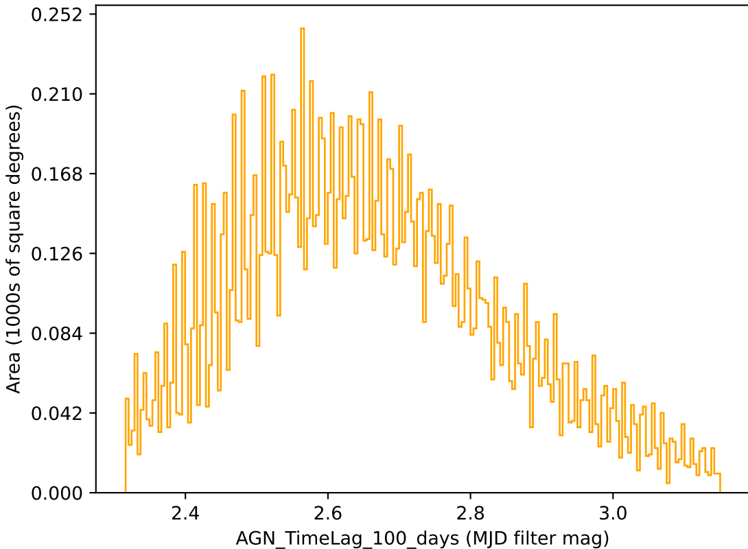
no_long_v3.4_10yrs r band: AGN_TimeLag_100_days
