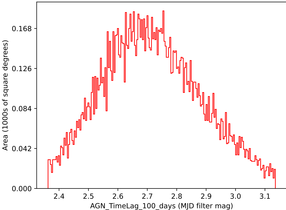
no_long_v3.4_10yrs i band: AGN_TimeLag_100_days
